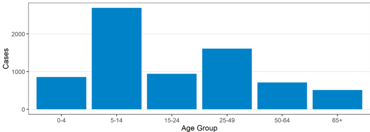
2022-2023 Influenza Season Case Age Distribution through January 21, 2023
