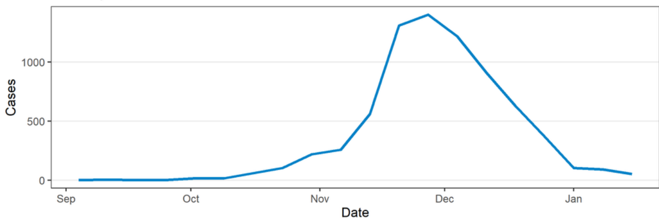
2022-2023 Influenza Cases Over Time in St. Charles County through January 21, 2023
