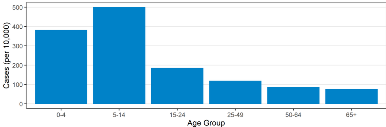
2022-2023 Influenza Season Age-Specific Case Rates through January 21, 2023
