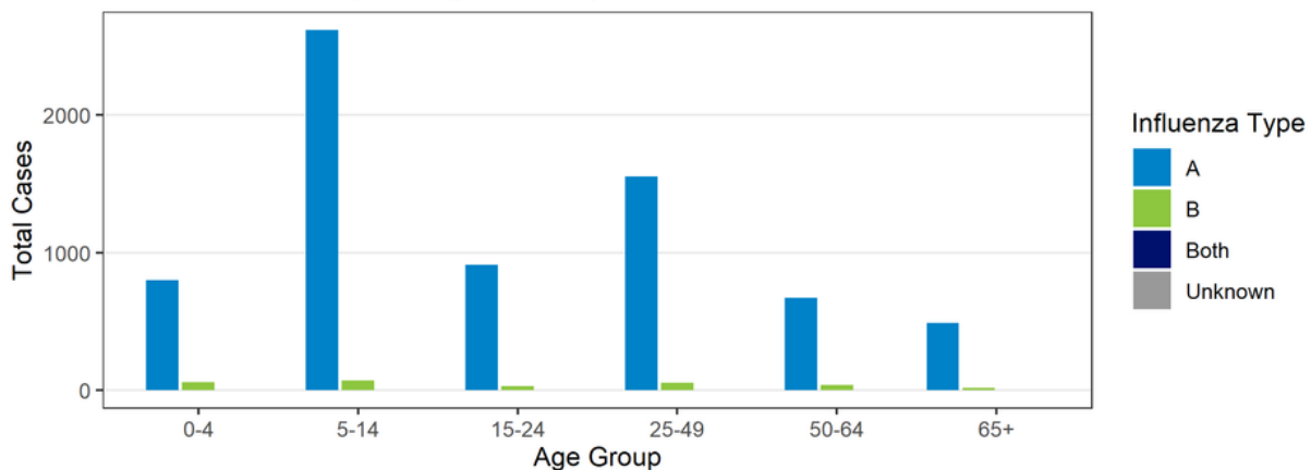
2022-2023 Influenza Season Cases by Age Group and Type in St. Charles County through January 21, 2023
