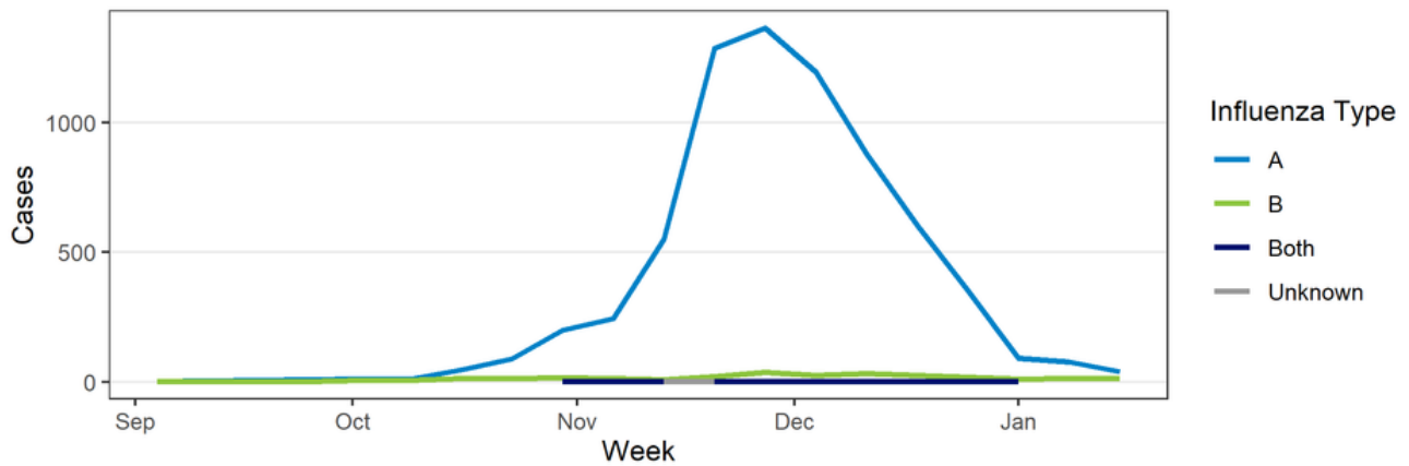
2022-2023 Influenza Season Case Type Over Time through January 21, 2023
