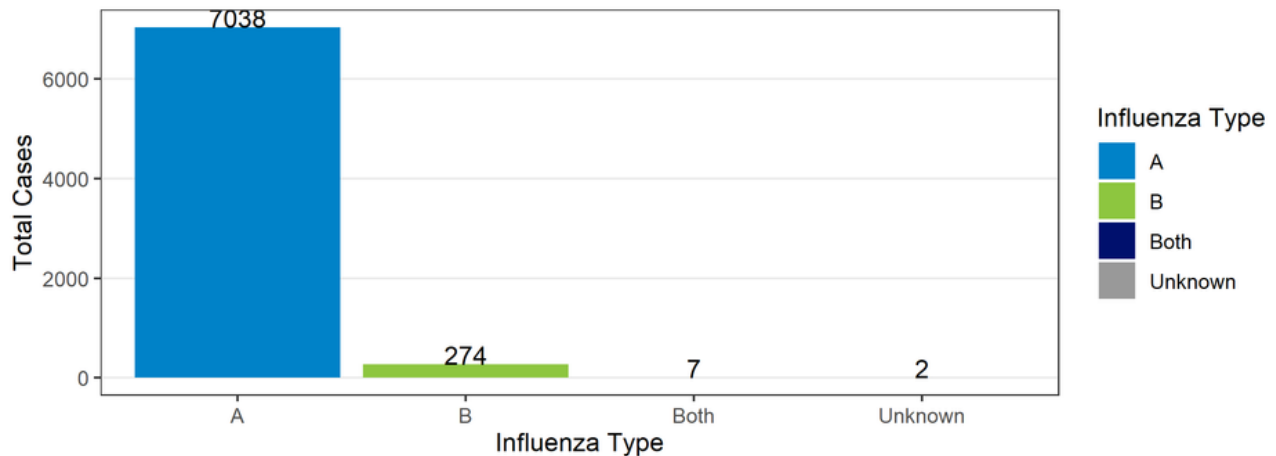
2022-2023 Influenza Season Cases by Type in St. Charles County through January 21, 2023
